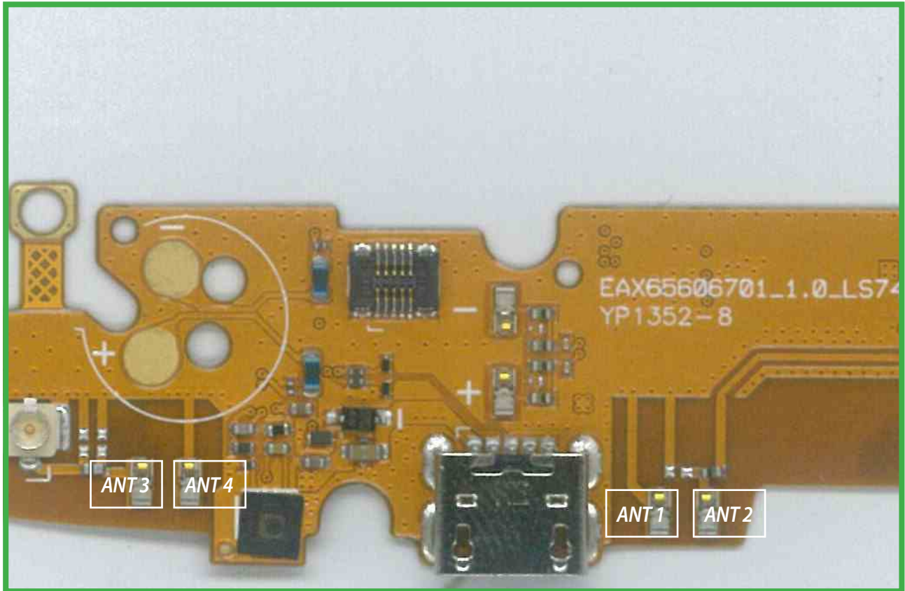
Lower FPCB (Bottom)
