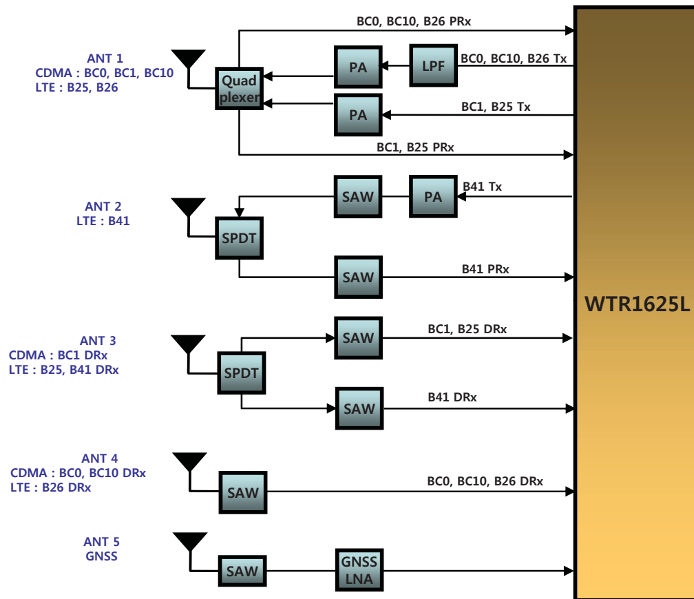
[LS740] RF_CDMA/LTE Block Diagram
