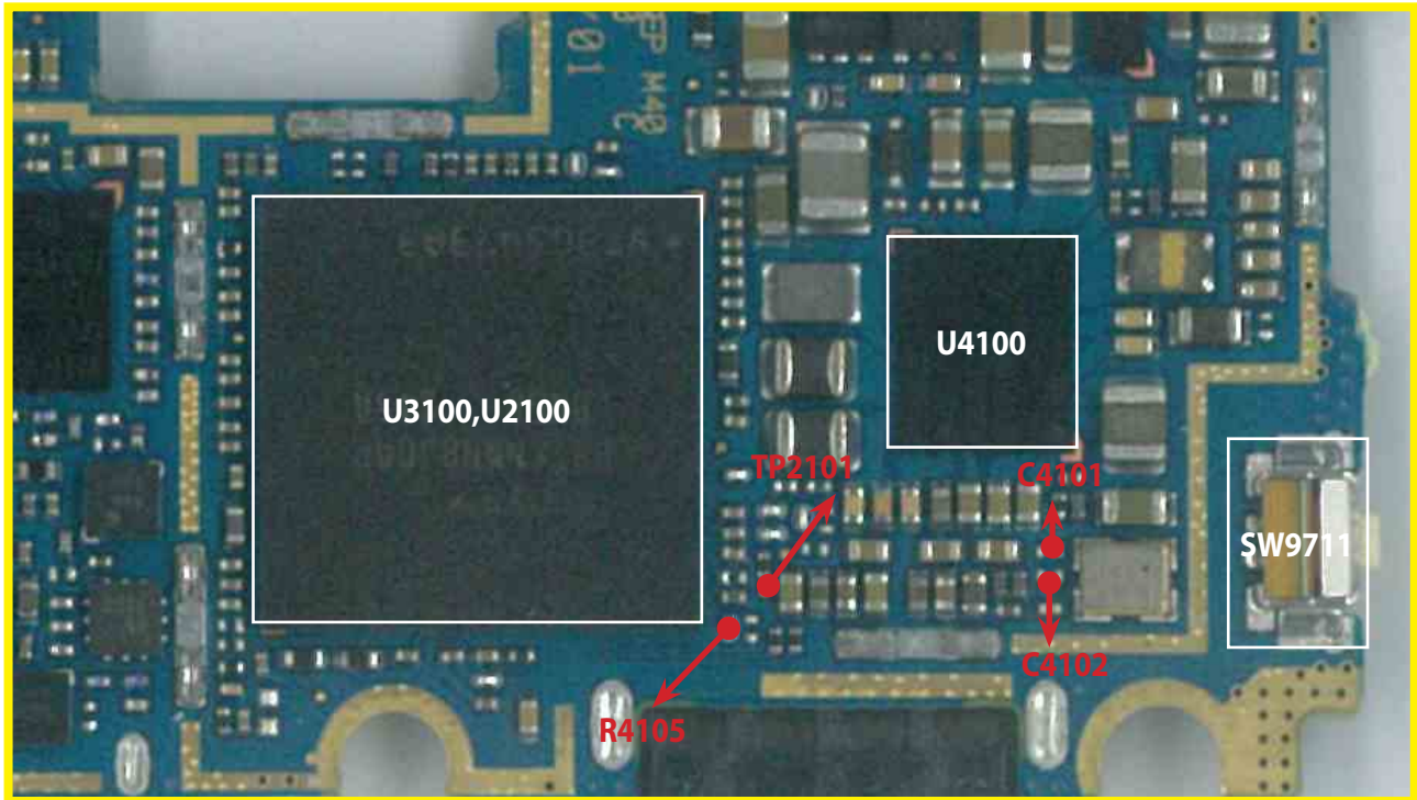
Power ON Troubleshooting (MSM8926)
