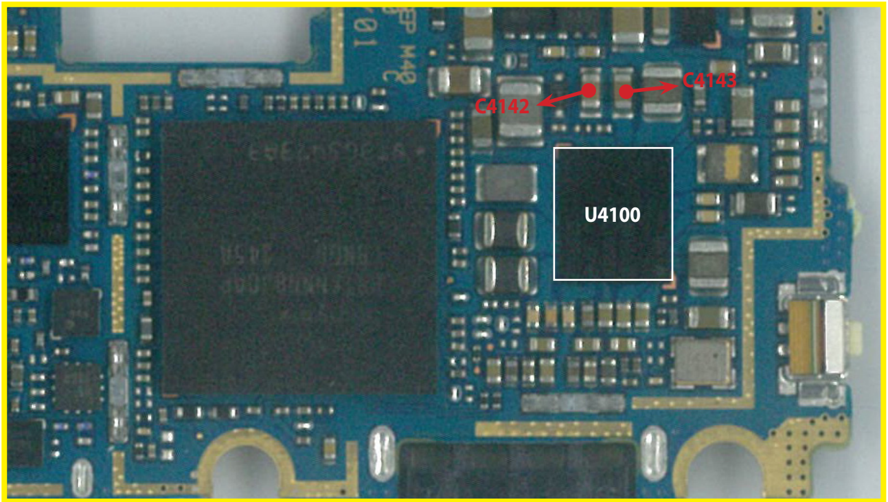
Charging Troubleshooting <Main Top>
