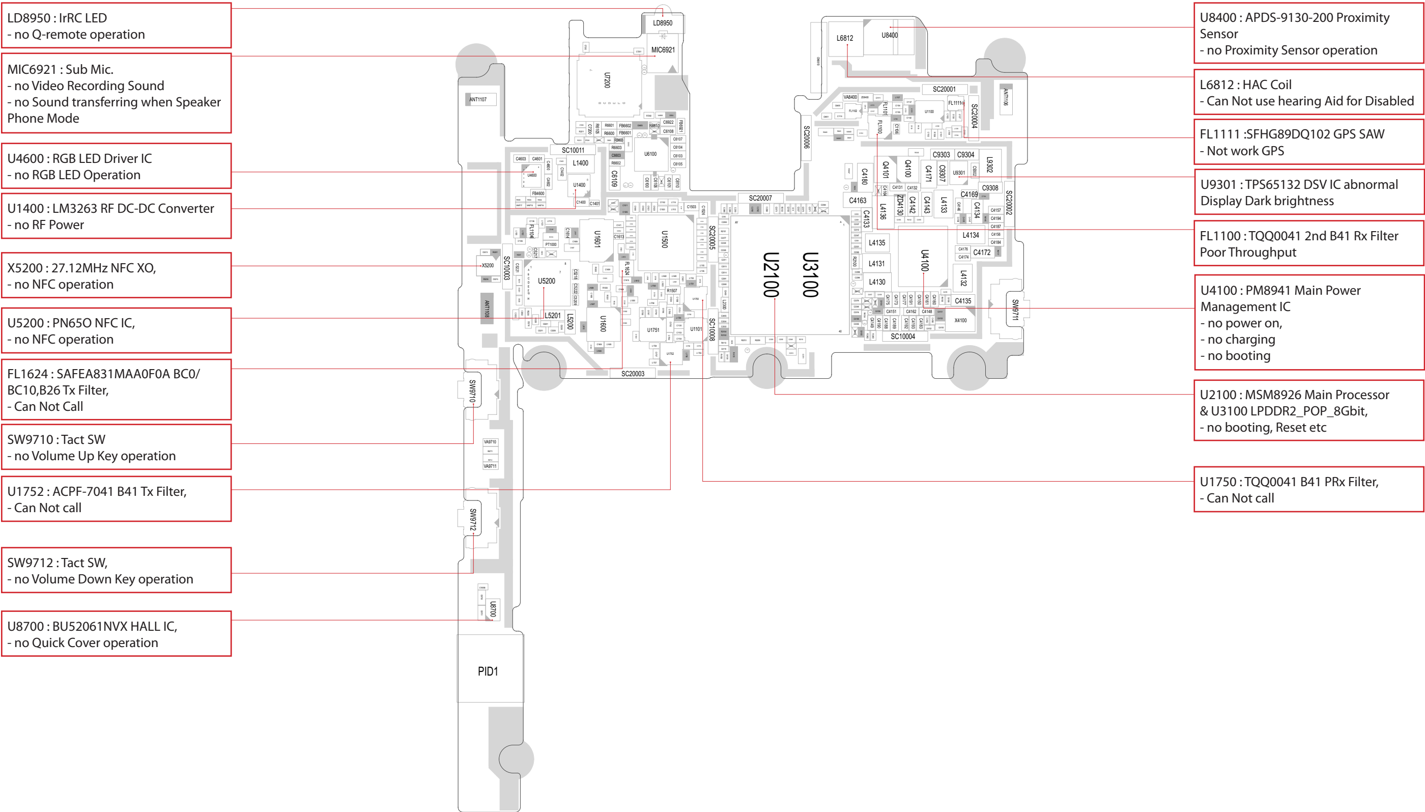
LG-LS740_MAIN_EAX65588701_1.0_TOP-1
