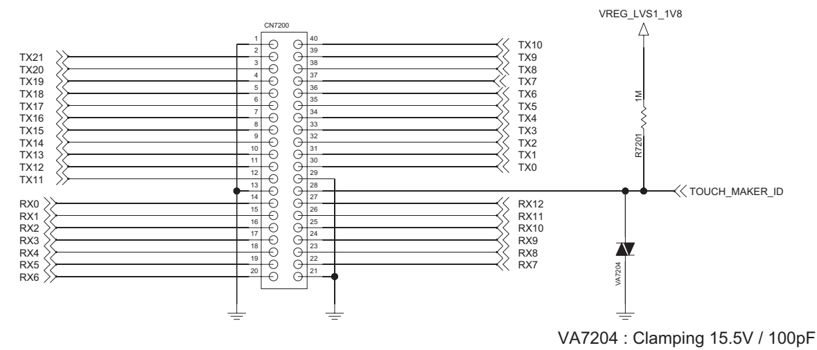
Touch Connector ( B to B type )
