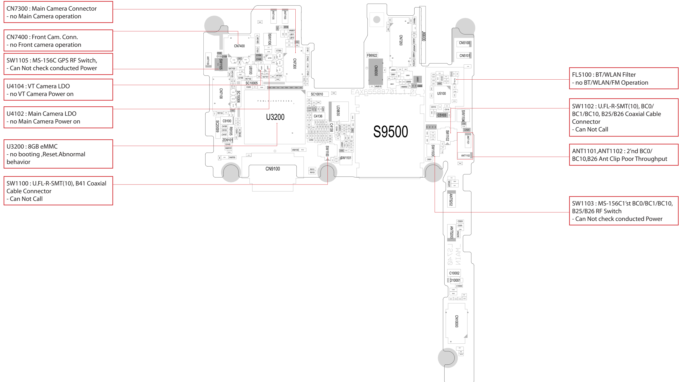
LG-LS740_MAIN_EAX65588701_1.0_BOT-2
